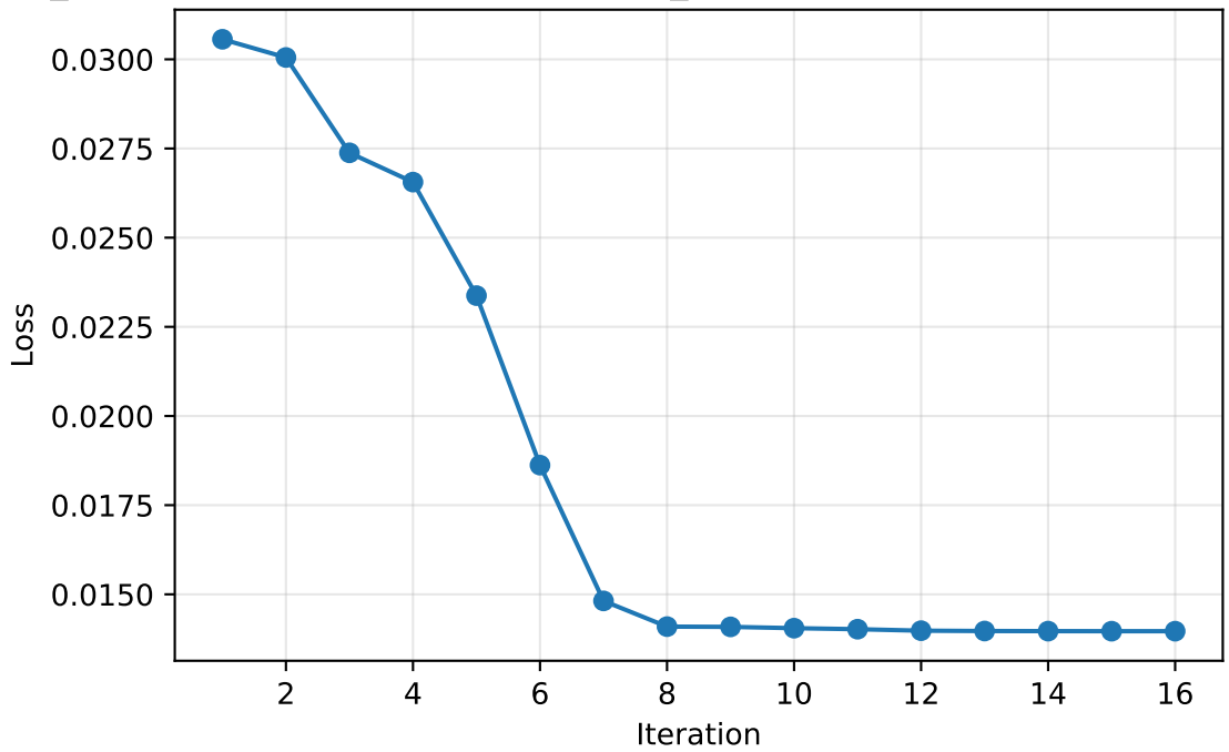
Loss curve | model=noisy_or, tying=4, agent=gpt-4, prompt_category=numeric-certainty, domain=None, ver=2, temp=0.0
