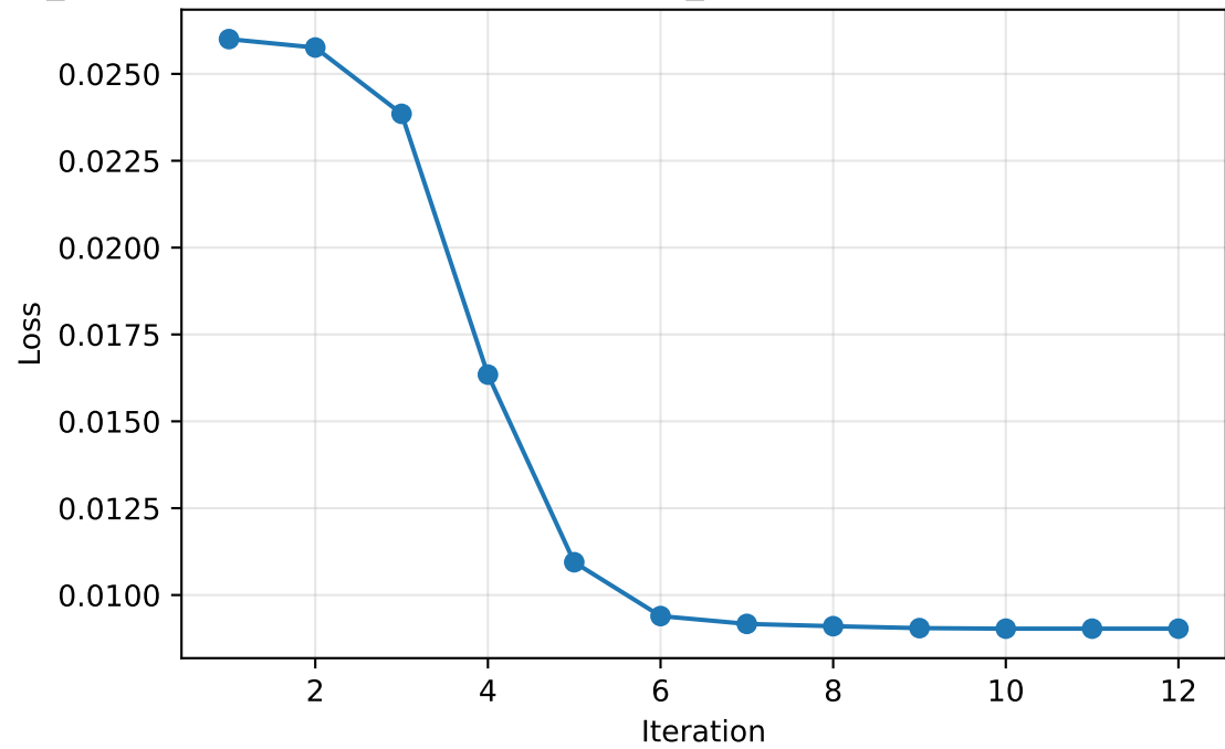
Loss curve | model=noisy_or, tying=3, agent=gpt-4o, prompt_category=numeric-certainty, domain=None, ver=2, temp=0.0
