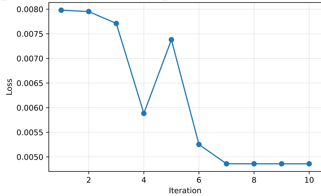
Loss curve | model=noisy_or, tying=3, agent=gpt-4, prompt_category=numeric-confidence-CoT, domain=None, ver=2, temp=0.0
