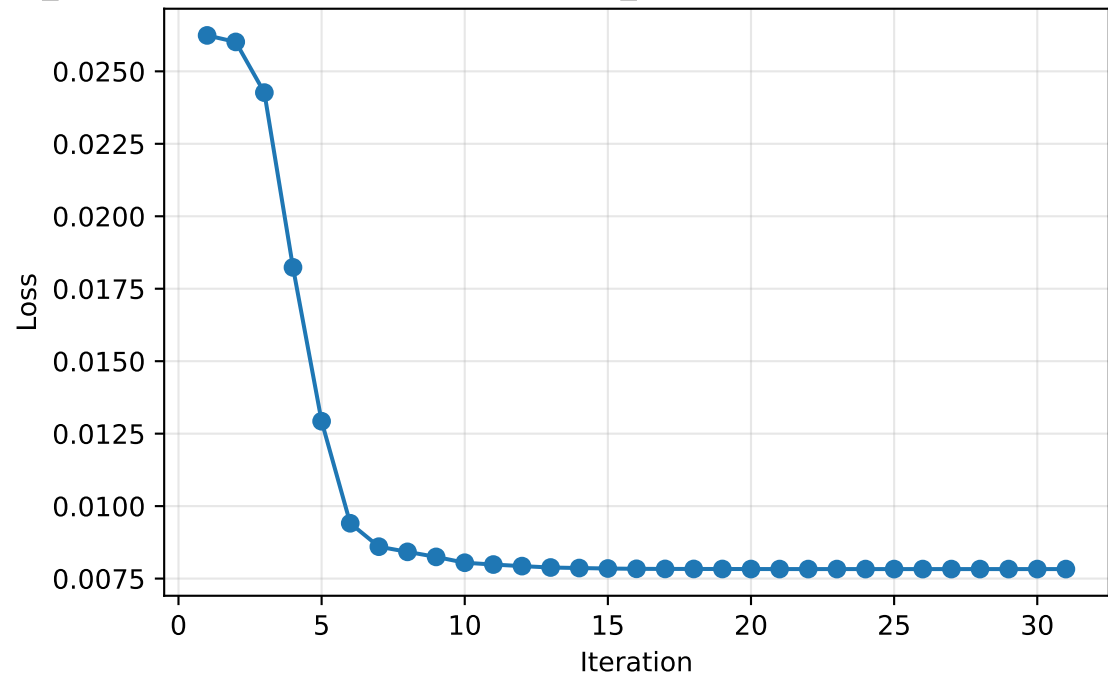
Loss curve | model=noisy_or, tying=5, agent=gpt-4o, prompt_category=numeric-certainty, domain=None, ver=2, temp=0.0
