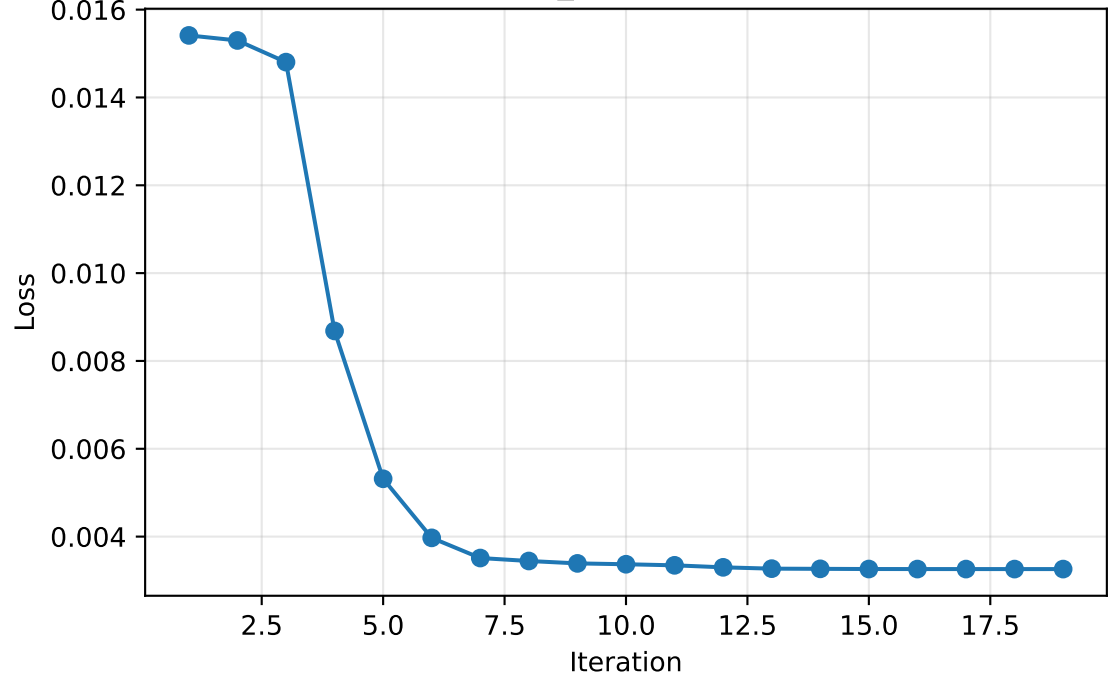
Loss curve | model=noisy_or, tying=5, agent=gpt-4o, prompt_category=numeric-confidence-CoT, domain=None, ver=2, temp=0.0
