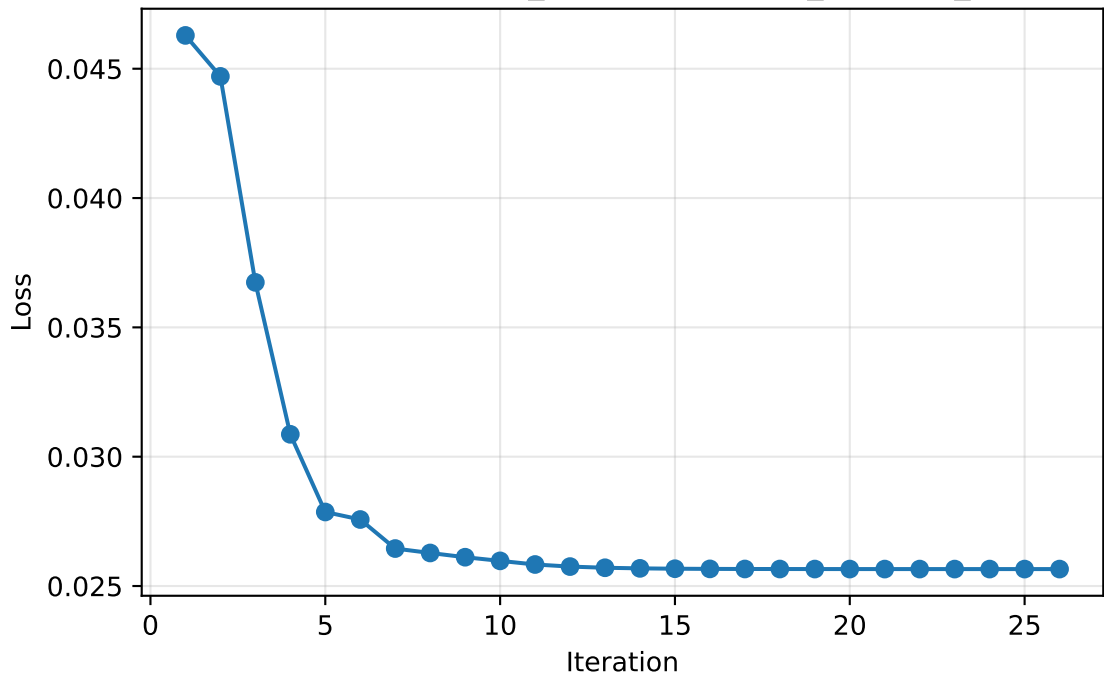
Loss curve | model=logistic, tying=4, agent=gpt-4, prompt_category=single_numeric_response, domain=None, ver=2, temp=0.0
