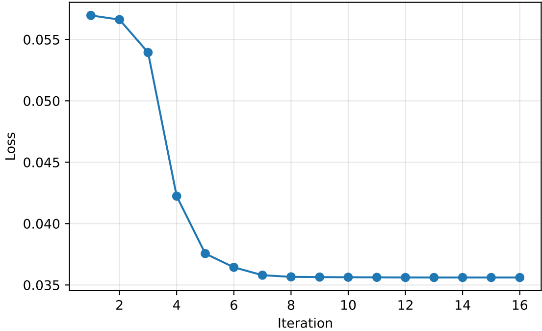
Loss curve | model=noisy_or, tying=5, agent=gpt-4.1-mini, prompt_category=numeric-certainty, domain=None, ver=2, temp=0.0
