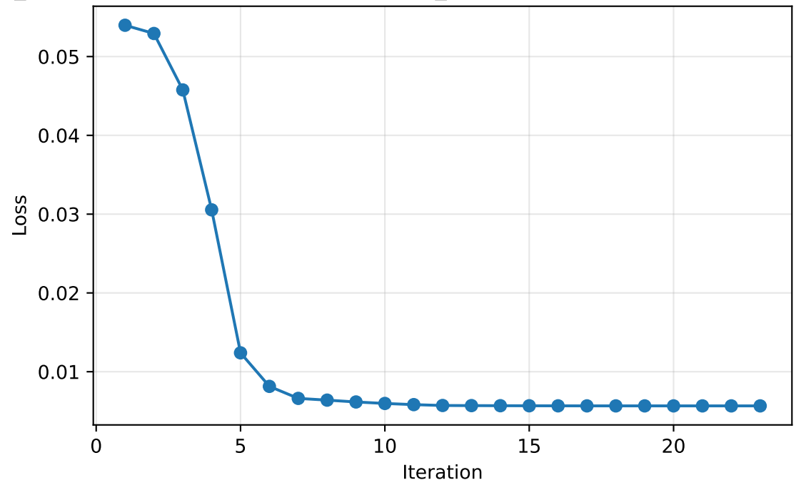
Loss curve | model=noisy_or, tying=5, agent=gpt-4.1, prompt_category=numeric-certainty, domain=None, ver=2, temp=0.0
