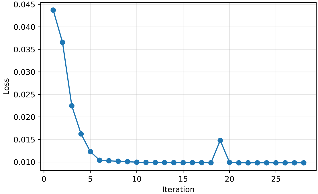
Loss curve | model=logistic, tying=4, agent=o3, prompt_category=numeric-confidence-CoT, domain=None, ver=2, temp=0.0
