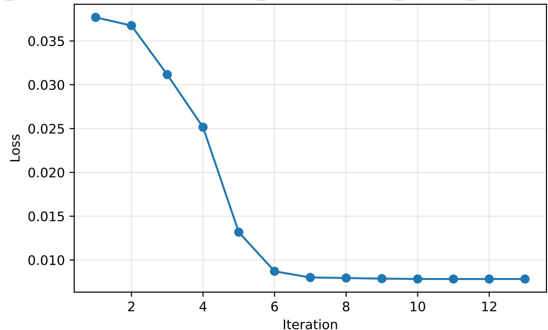
Loss curve | model=noisy_or, tying=5, agent=o3, prompt_category=single_numeric_response, domain=None, ver=2, temp=0.0
