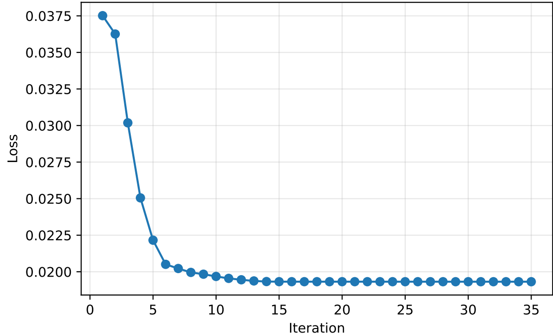
Loss curve | model=logistic, tying=5, agent=gpt-4, prompt_category=numeric-certainty, domain=None, ver=2, temp=0.0
