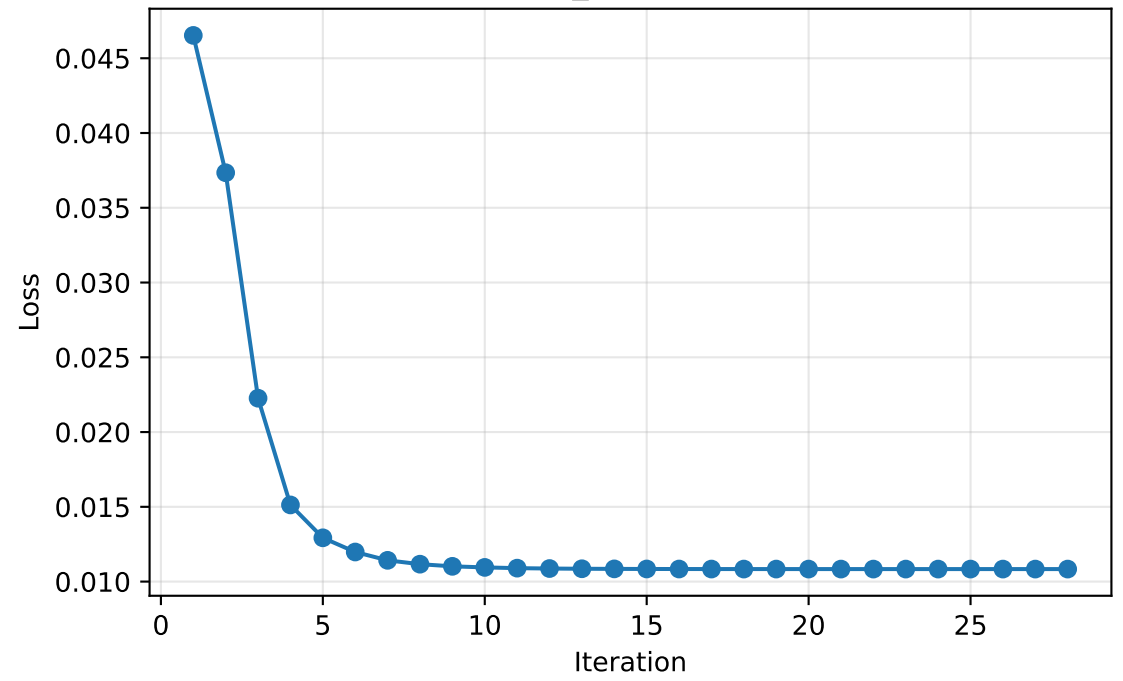
Loss curve | model=logistic, tying=3, agent=o3, prompt_category=numeric-certainty, domain=None, ver=2, temp=0.0
