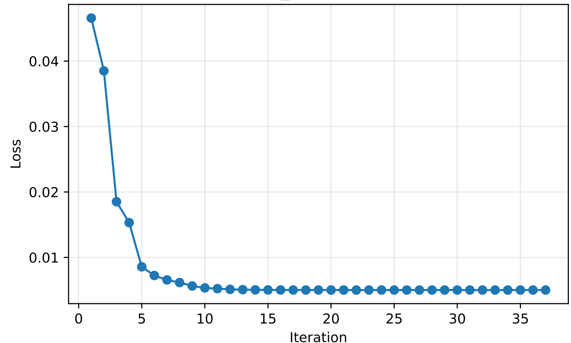
Loss curve | model=logistic, tying=4, agent=gpt-4.1, prompt_category=numeric-confidence-CoT, domain=None, ver=2, temp=0.0
