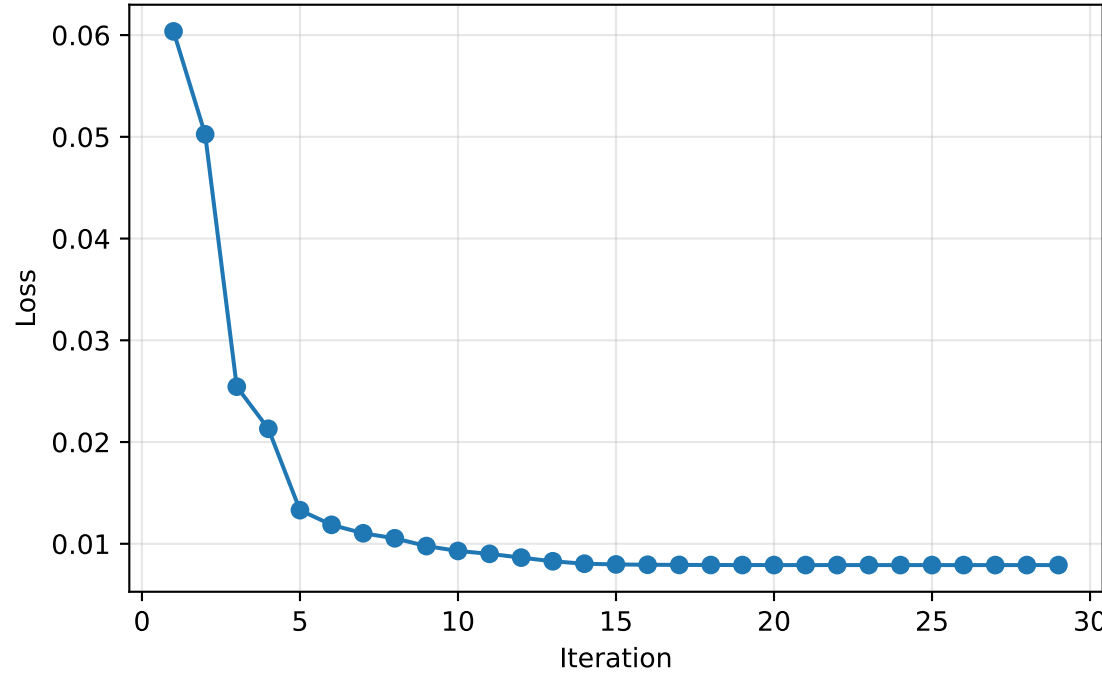
Loss curve | model=logistic, tying=5, agent=gpt-4.1, prompt_category=single_numeric_response, domain=None, ver=2, temp=0.0
