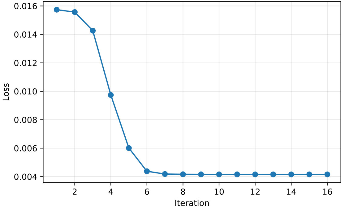
Loss curve | model=noisy_or, tying=5, agent=o3, prompt_category=numeric-certainty, domain=None, ver=2, temp=0.0
