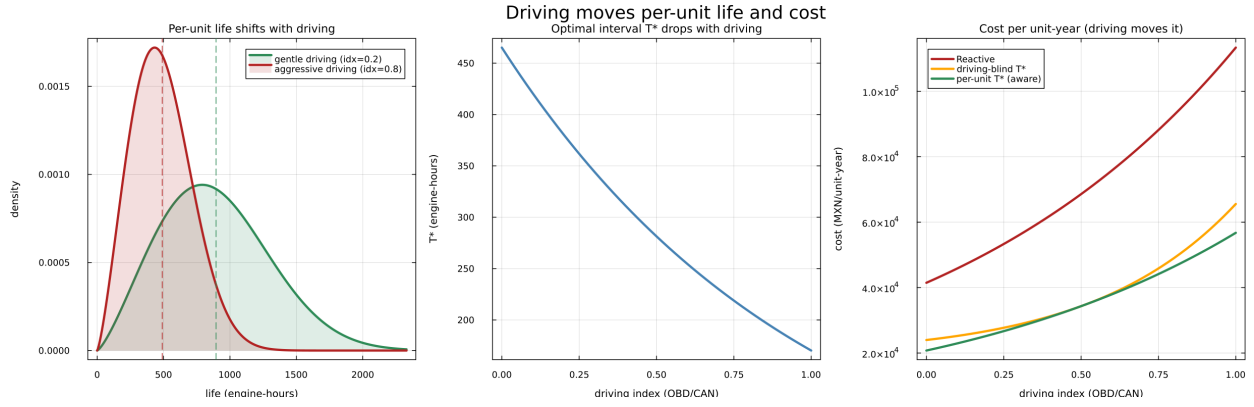
Figure 6: Driving moves per-unit life and cost. Left: the brake-pad life distribution shifts left under aggressive driving (the part dies younger). Center: the optimal interval T^* falls monotonically with the driving index. Right: cost per unit-year rises with driving; a driving-aware T^* (per unit) stays below a blind one (scheduled at an average interval). The driving index is derived from OBD/CAN telemetry. PhAIMaT simulation.
