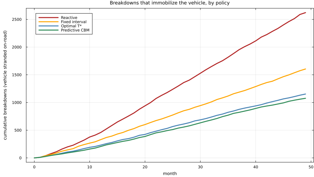
Figure 3: Breakdowns that immobilize the vehicle (on-road failure), accumulated by policy. Output of PhAIMaT’s agent-physical simulator over a 60-truck fleet across 4 years: reactive accumulates 2,622 immobilizations; predictive CBM, 1,076. Each is a c_{\text{breakdown}} event —roadside repair, emergency premium and stopped time.
