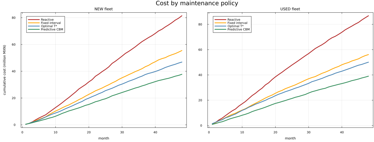
Figure 4: Cumulative cost by policy , for new (dealer) and used fleets. The optimal T^* and predictive CBM clearly separate from reactive and fixed-interval; on a new fleet the predictive closes at 37.7 M MXN versus 81.4 M for reactive (4 years, 60 trucks). PhAIMaT simulation .
