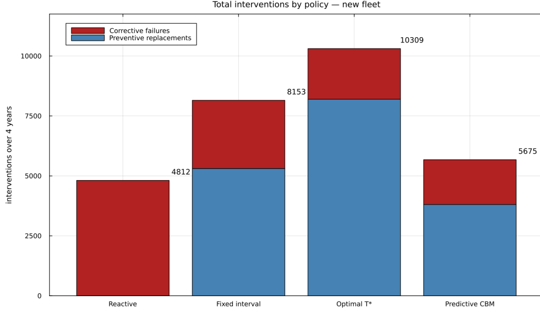
Figure 5: Total interventions by policy. T^* and CBM achieve similar safety (corrective failures 2,112 vs 1,869), but T^* makes 8,197 preventive replacements against 3,806 for CBM: same protection, far more over-maintenance. It is the difference the cost curve (Figure 4) translates into ~20 % savings of CBM over T^* . PhAIMaT simulation.
