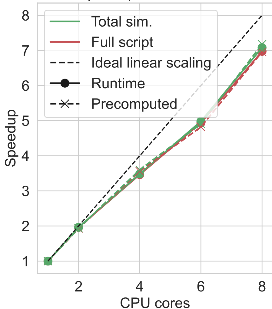
Speedup vs CPU Cores
