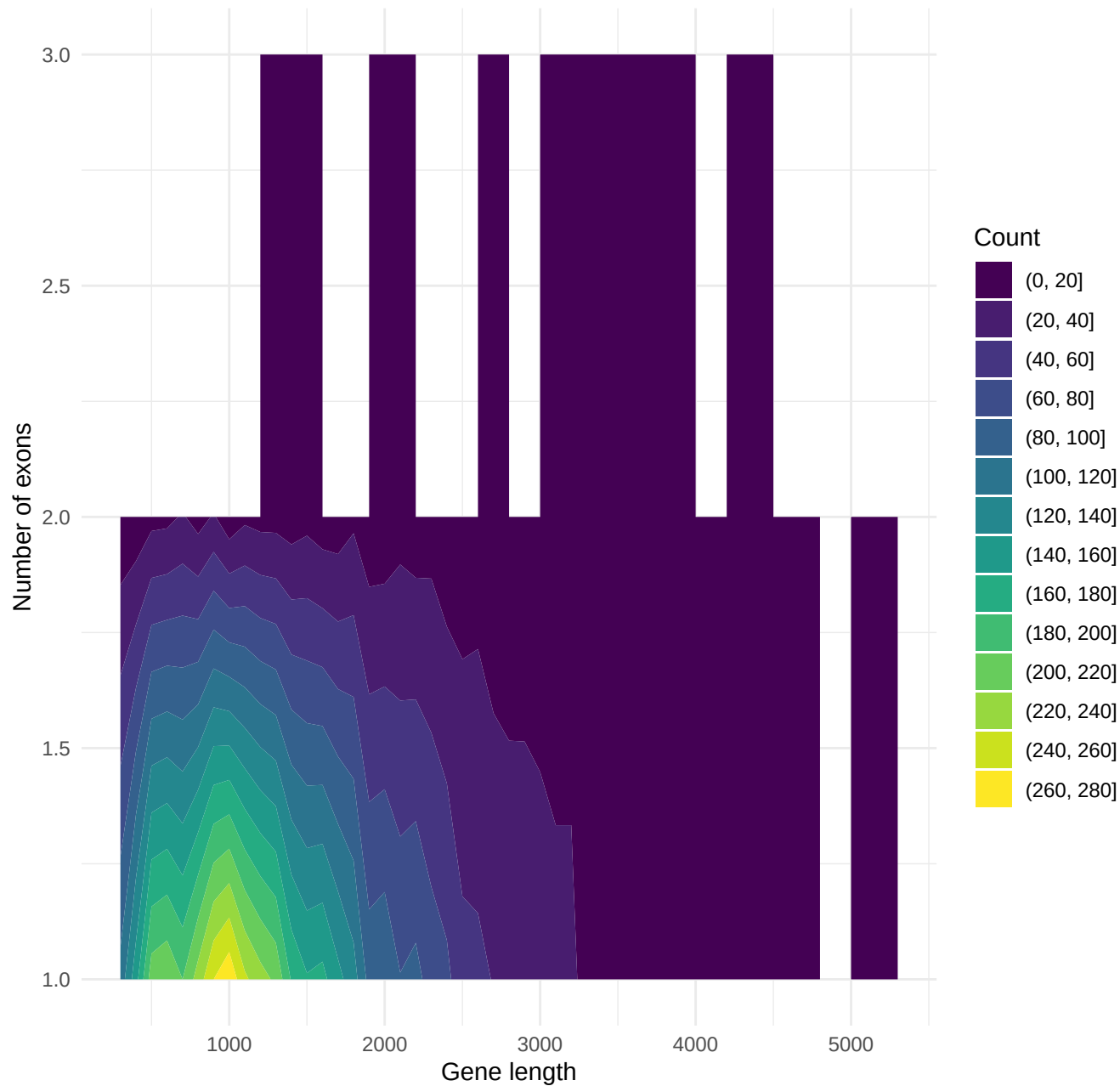
Contour Map of gene_len vs num_exons
