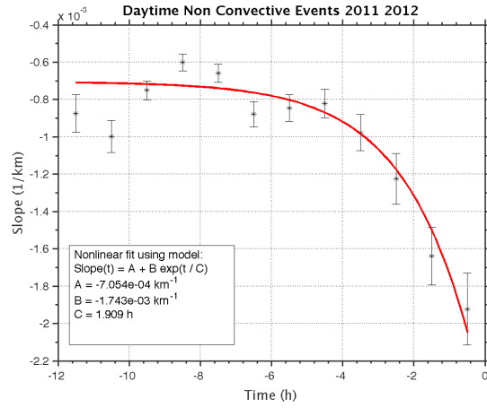
Daytime Non Convective Events 2011 2012 averaged over events, lines = statio Daytime Non Convective Events 2011 2012 averaged over stations, lines = ever
