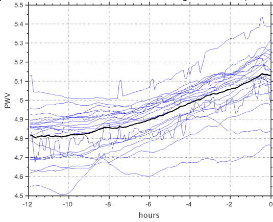
Daytime Non Convective Events 2011 2012 averaged over events, lines = statio Daytime Non Convective Events 2011 2012 averaged over stations, lines = ever
