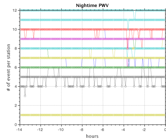
Figure 3: Nighttime_PWV_14hr_interval_2011_2012.dat, ntimes=168, nevents=12, nstation=21, max dist=150, file dt=5
