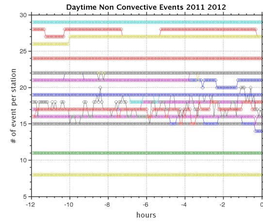
Figure 10: Daytime_Non_Convective_Events.2011_2012.12hr_interval_output.dat, ntimes=144, nevents=30, nstation=21, max dist=150, file dt=5
