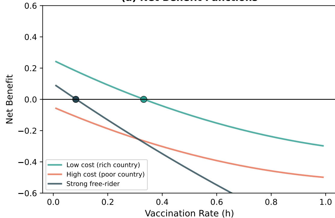
(a) Net Benefit Functions
