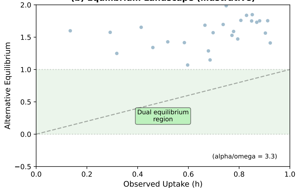
(b) Equilibrium Landscape (illustrative)
