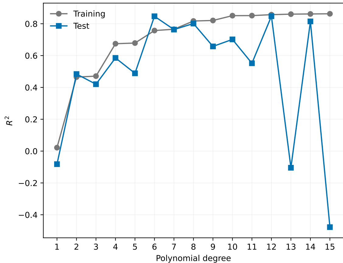
OLS R^2 ( N = 100, \sigma = 0.1 )
