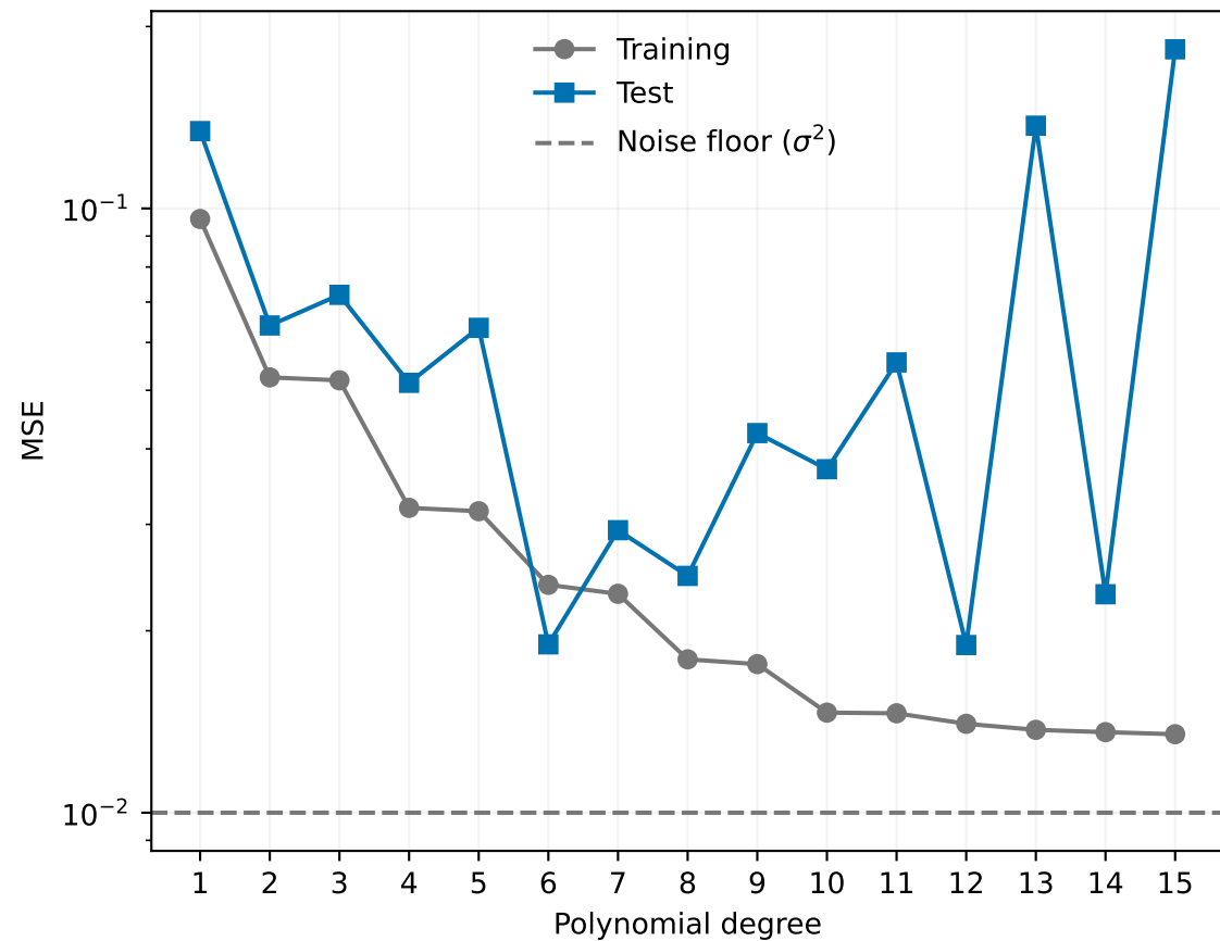
OLS MSE ( N = 100, \sigma = 0.1 )
