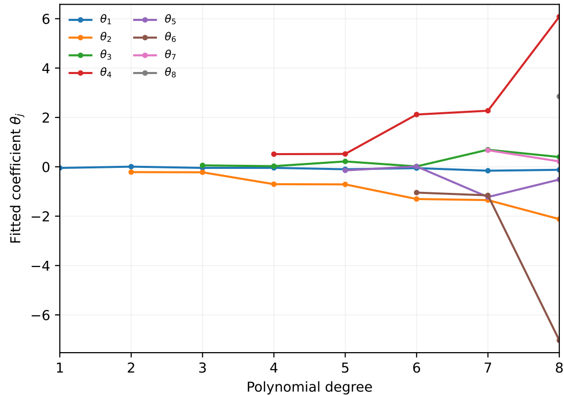
Polynomial degrees 1-8
