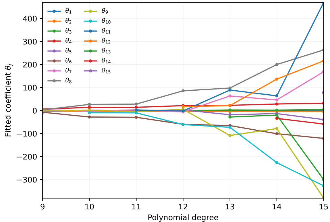
Polynomial degrees 9-15
