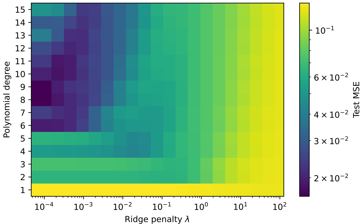
Ridge test MSE as a function of degree and \lambda
