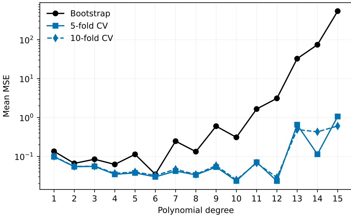
OLS error estimates: bootstrap vs. cross-validation
