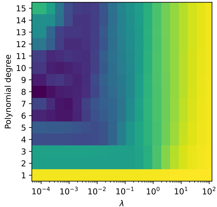
5-fold Ridge CV
