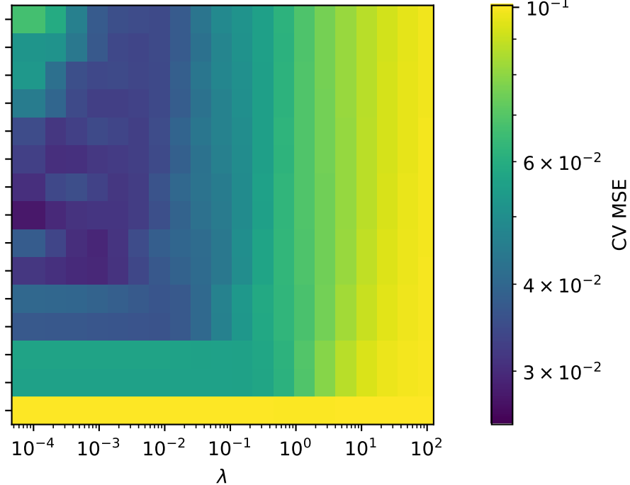
10-fold Ridge CV
