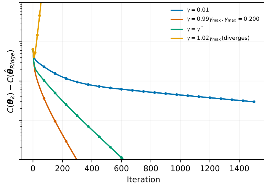
Ridge ( \lambda = 0.01 ), \kappa = 499.53
