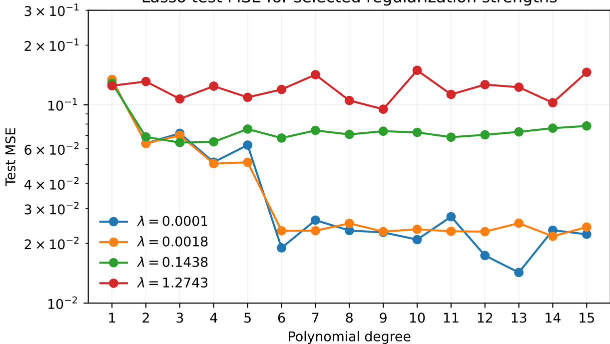
Lasso test MSE for selected regularization strengths
