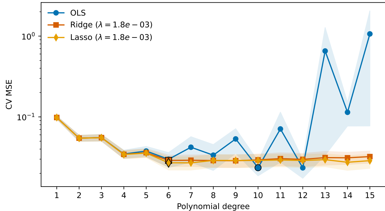
Five-fold cross-validation with one-standard-error bands
