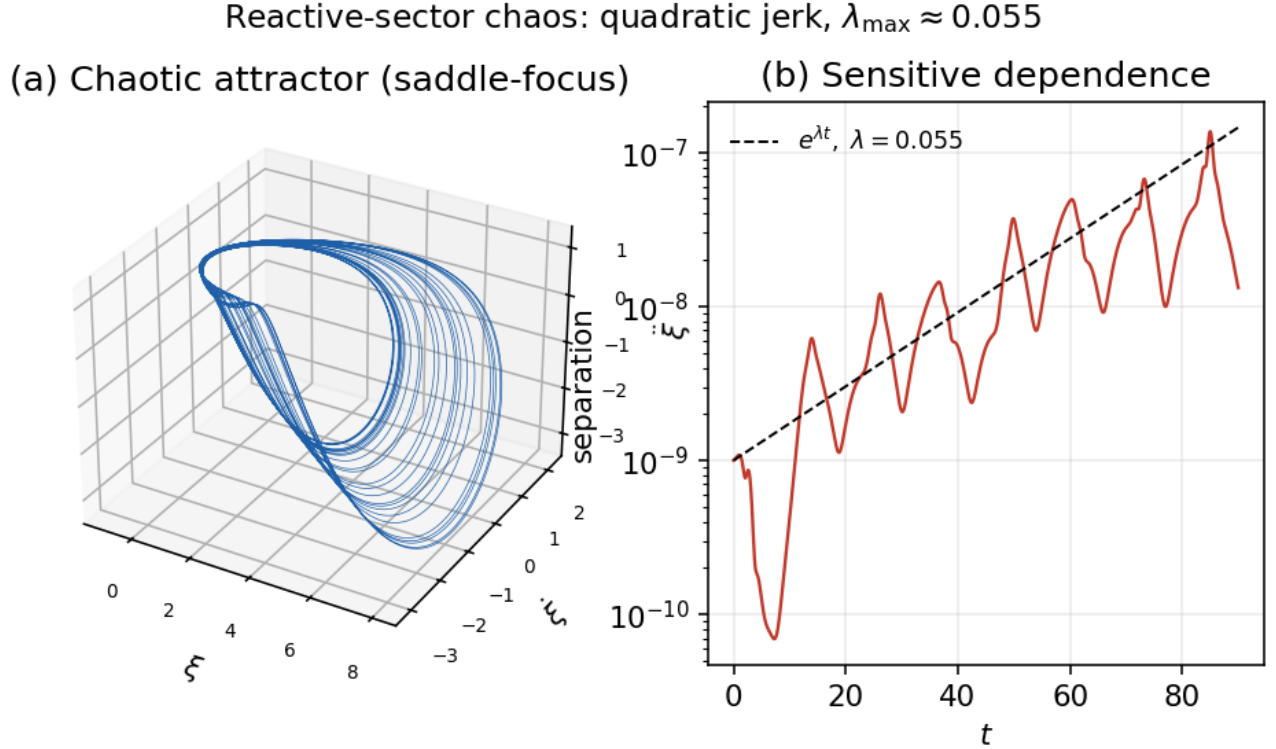
Figure 4: Figure 4. (a) Shilnikov-type chaotic attractor (saddle-focus) of the quadratic jerk equation. (b) Sensitive dependence: the separation of two trajectories grows as e^{\lambda t} with \lambda \approx 0.055 .
