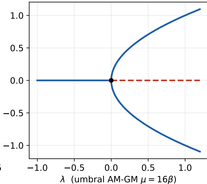
(b) Tridente (pitchfork) \dot{\xi} = \lambda\xi - \xi^3
