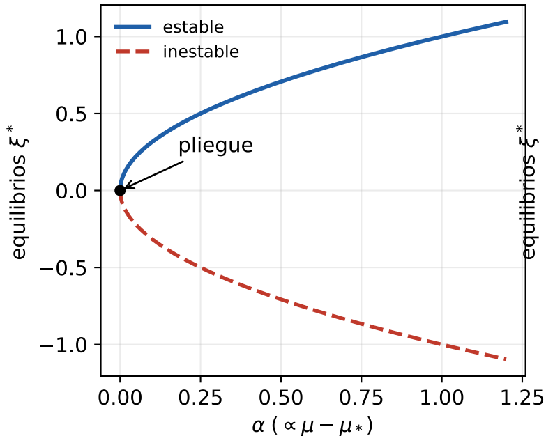
(a) Pliegue (saddle-node) \dot{\xi} = \alpha - \xi^2
