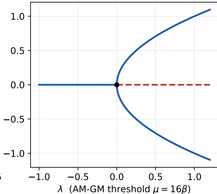
(b) Pitchfork \dot{\xi} = \lambda \xi - \xi^3
