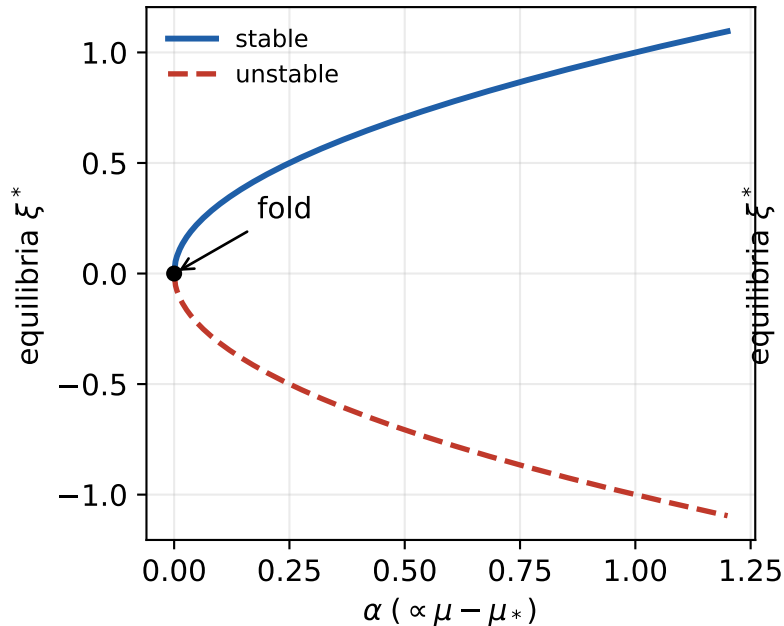
(a) Fold (saddle-node) \dot{\xi} = \alpha - \xi^2
