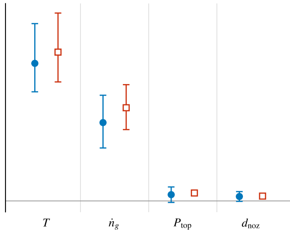
optimistic (Malinauskas K_s , Fukada D_l )
