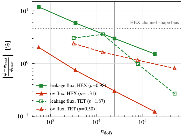
(a) discretization error HEX, refinement 1
