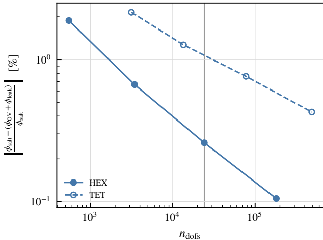
(b) mass conservation HEX, refinement 1
