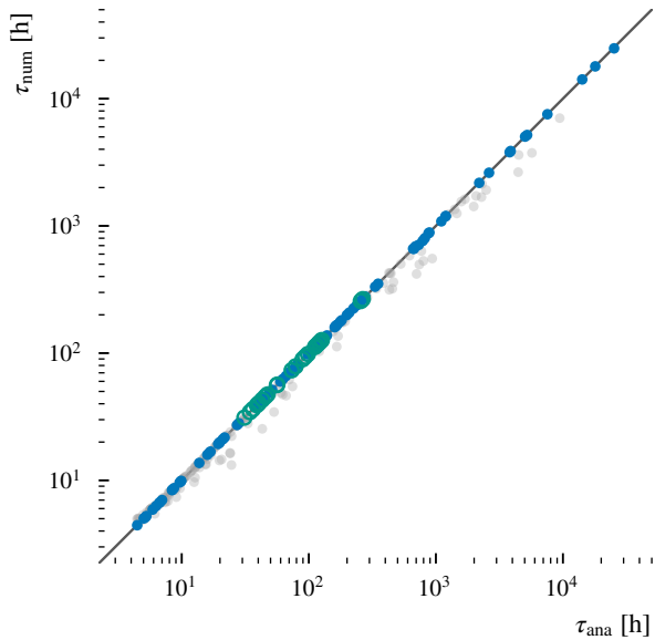
(a) parity
