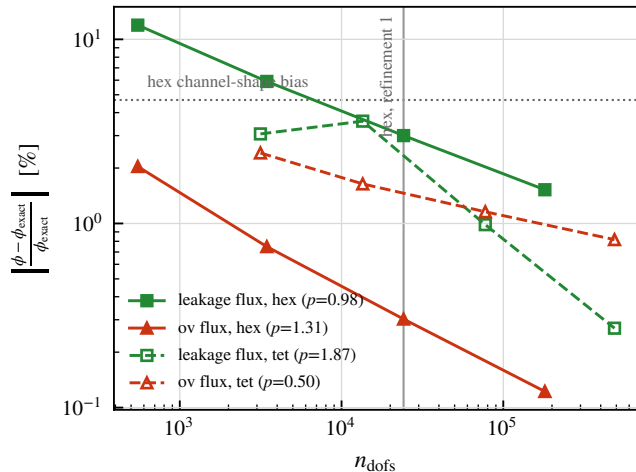
(a) discretization error
