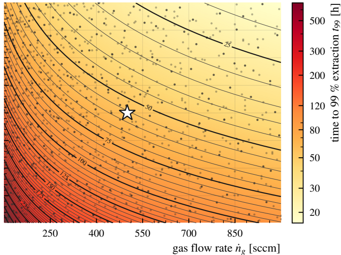
optimistic (Malinauskas K_s , Fukada D_l ) contour interval 25 h (5 h intermediate)
