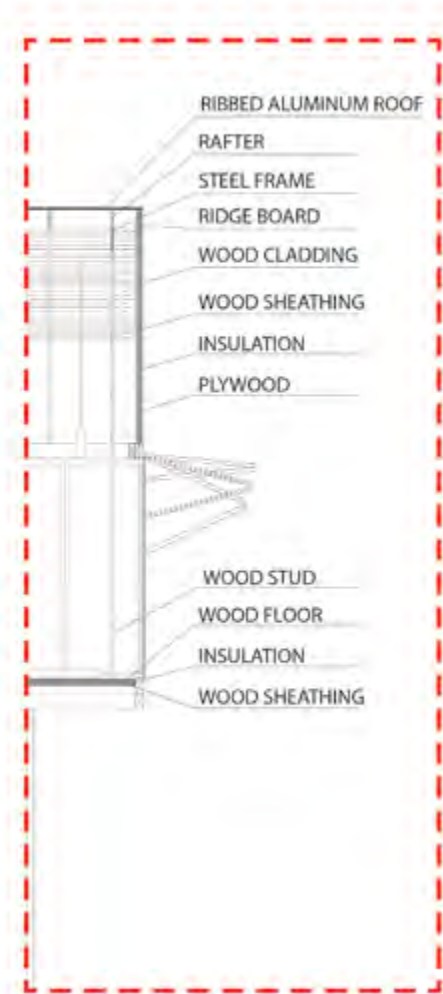
Detailed Section
