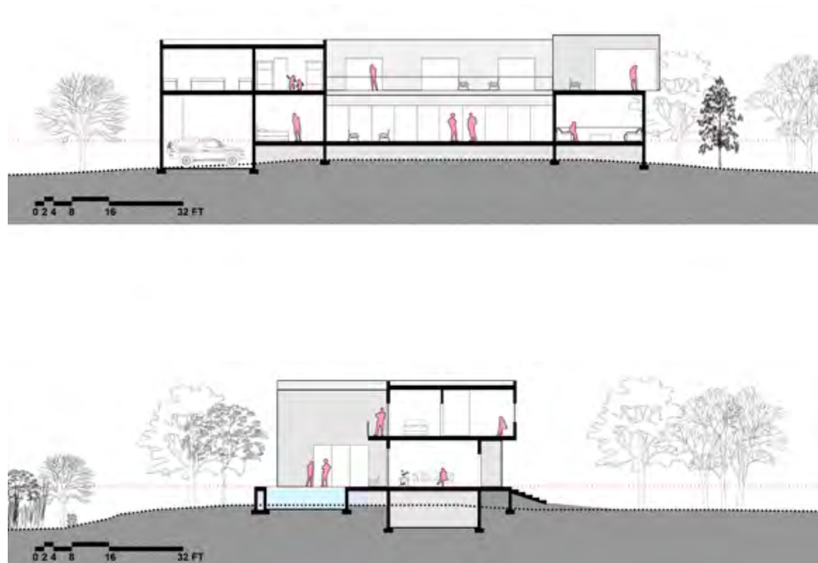
Sections
