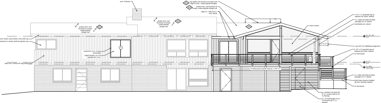
West Elevation
