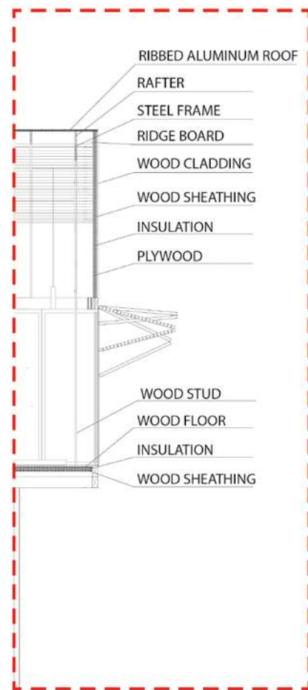
Detailed Section
