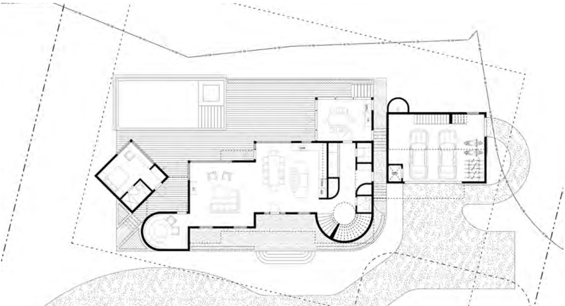
First Floor
