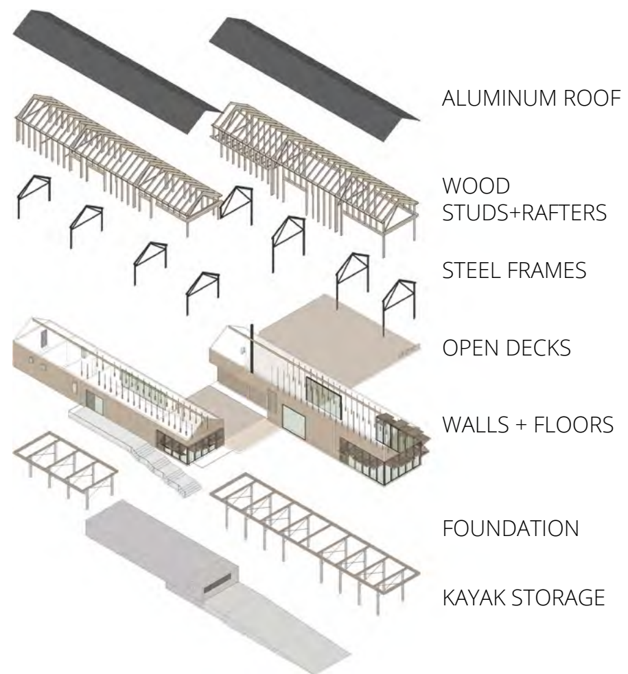
Structural Axon
