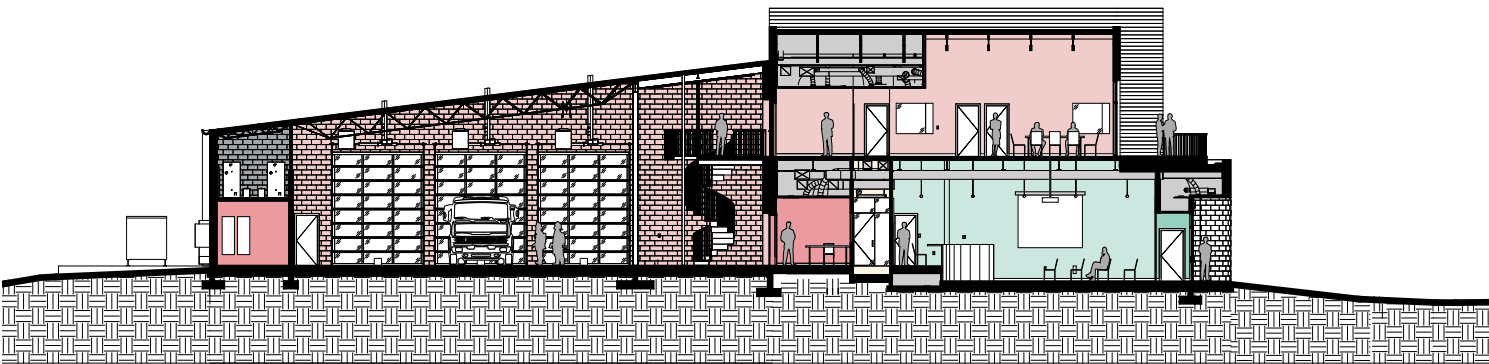
North Section
