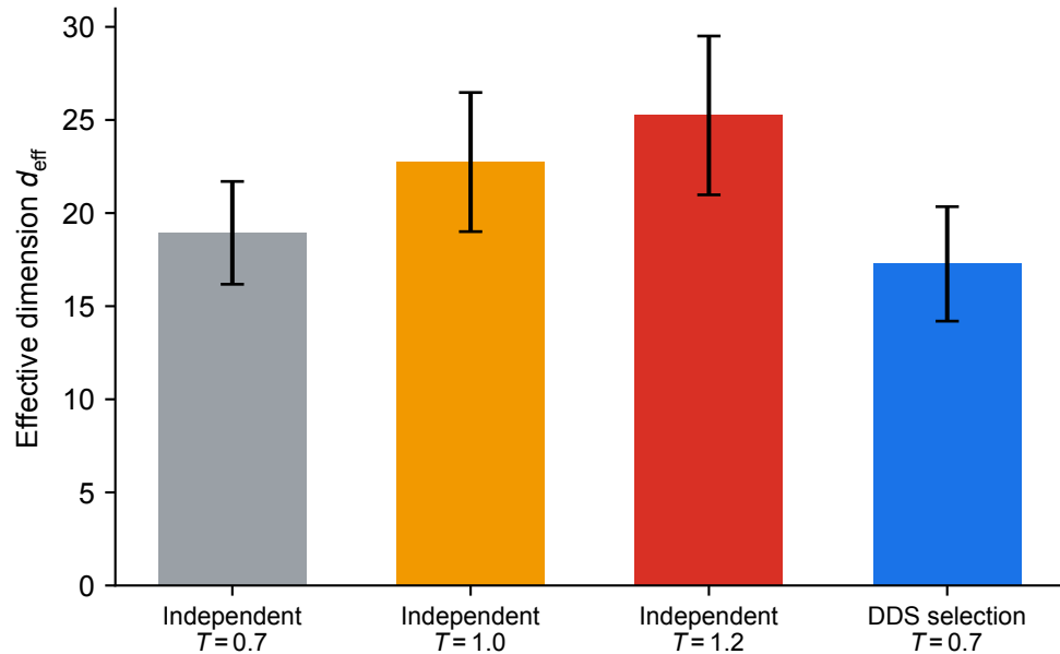
(a) Effective dimension (matched n = 120 )
