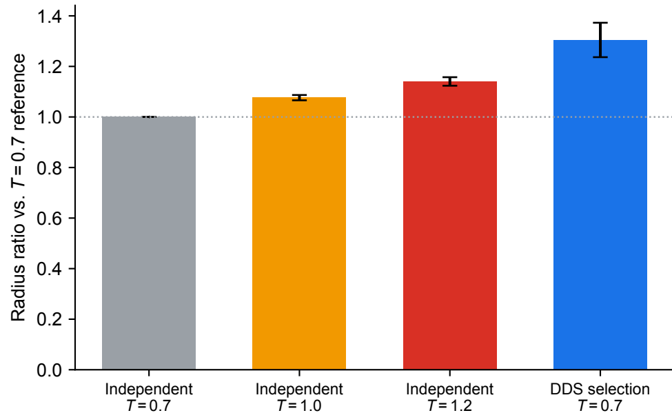
(b) Mean radius from the T=0.7 centroid
