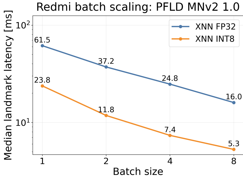
■ Figure 5.5 Landmark-inference latency batch scaling on Redmi for PFLD-MNv2-1.0 using XNNPACK variants. Lower latency is better.
