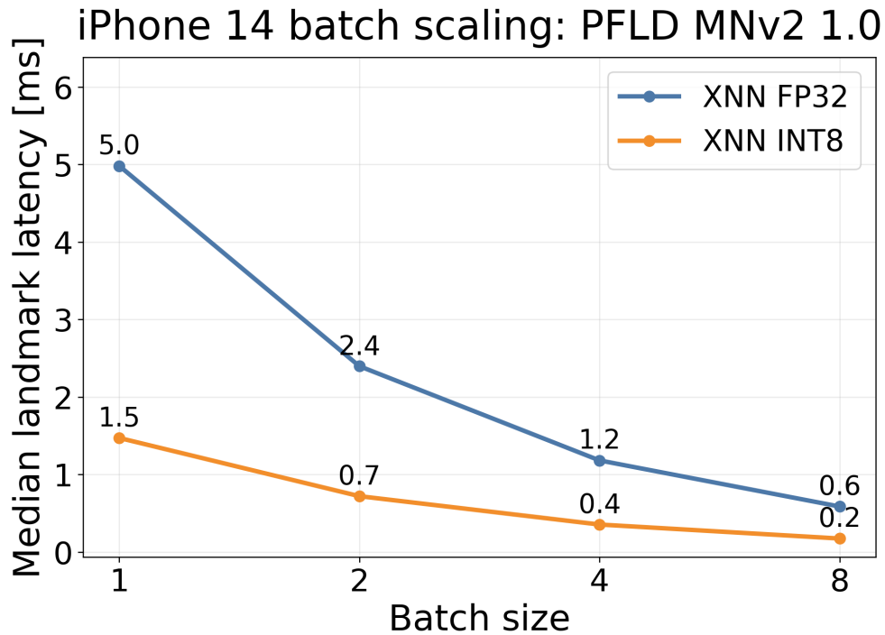
■ Figure 5.11 Landmark-inference latency batch scaling on iPhone 14 for PFLD-MNv2-1.0.
