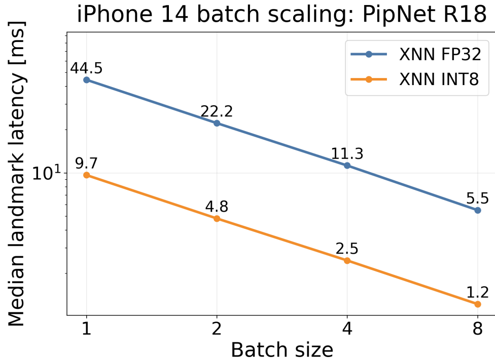
■ Figure 5.12 Landmark-inference latency batch scaling on iPhone 14 for PipNet ResNet18.
