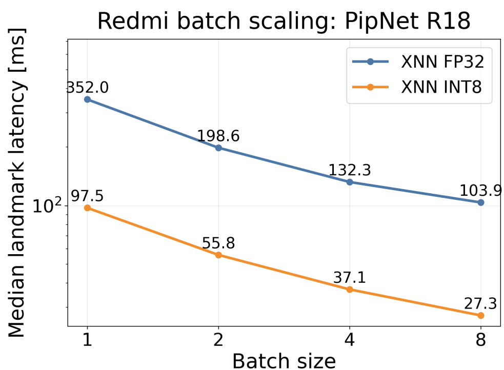
■ Figure 5.6 Landmark-inference latency batch scaling on Redmi for PipNet ResNet18 using XNNPACK variants. Lower latency is better.
