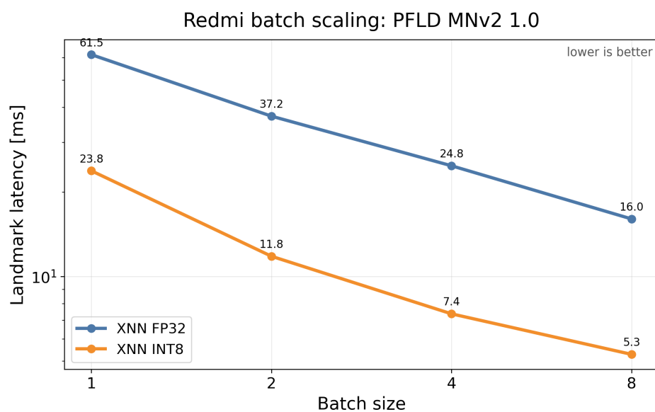
■ Figure 5.5 Redmi landmark-inference latency batch scaling for PFLD-MNv2-1.0 using XNNPACK variants. Lower latency is better.
