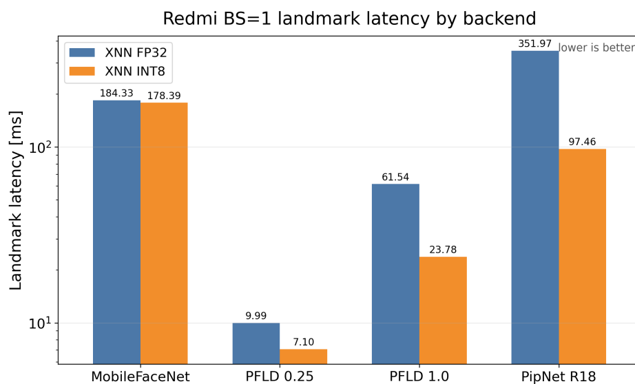
■ Figure 5.3 Redmi: BS=1 landmark-inference latency by backend and quantization. This chart focuses on the landmark model forward pass; lower latency is better.
