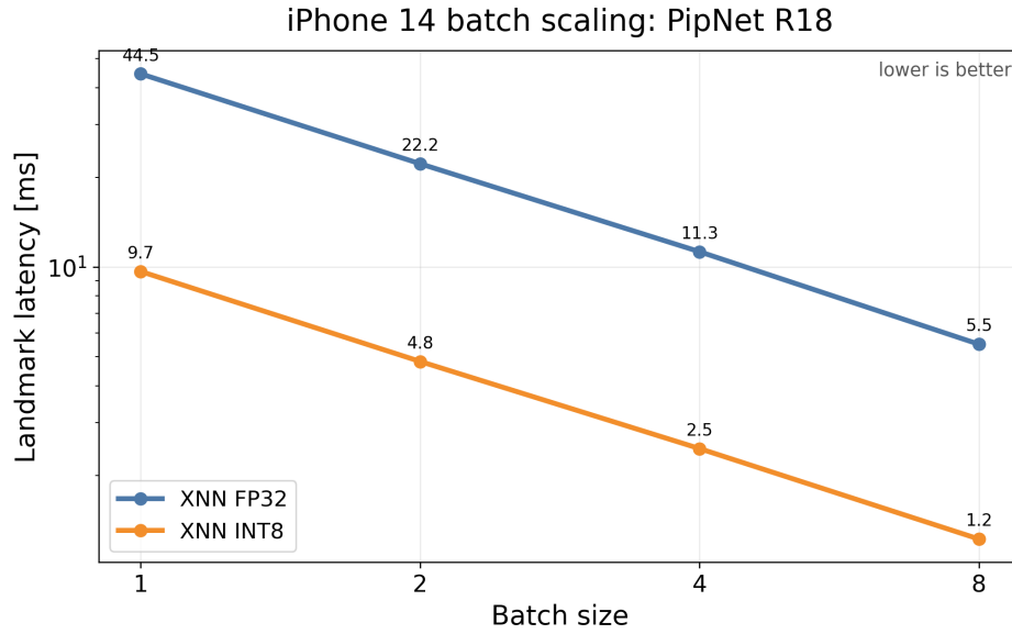
■ Figure 5.12 iPhone 14 landmark-inference latency batch scaling for PipNet ResNet18.
