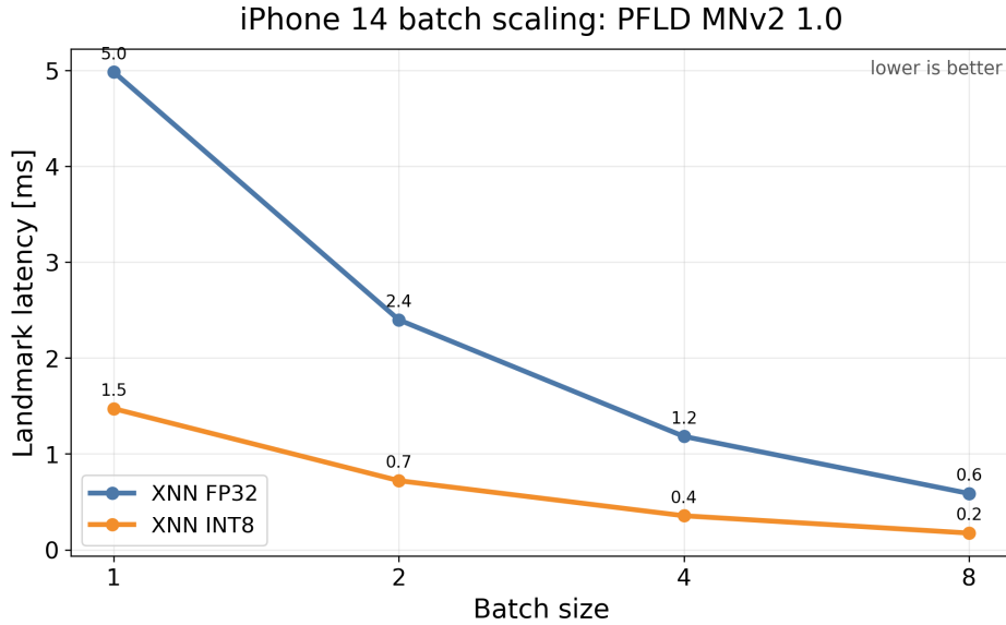
■ Figure 5.11 iPhone 14 landmark-inference latency batch scaling for PFLD-MNv2-1.0.
