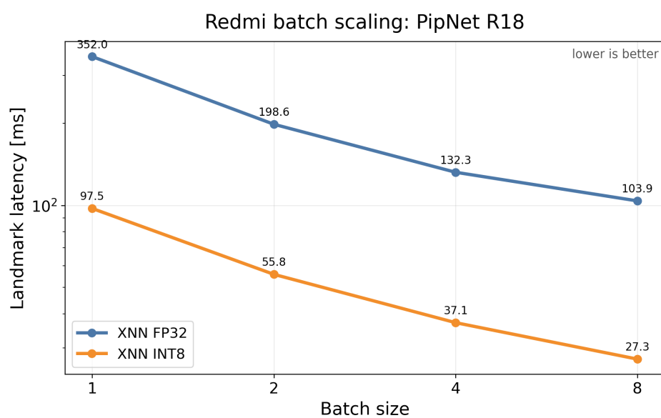
■ Figure 5.6 Redmi landmark-inference latency batch scaling for PipNet ResNet18 using XNNPACK variants. Lower latency is better.
