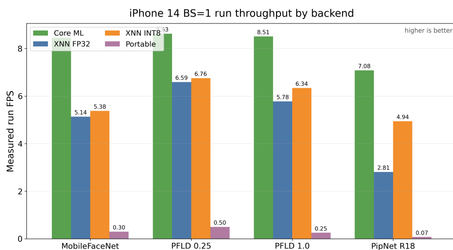
■ Figure 5.14 iPhone 14: BS=1 measured run throughput by backend and quantization.
