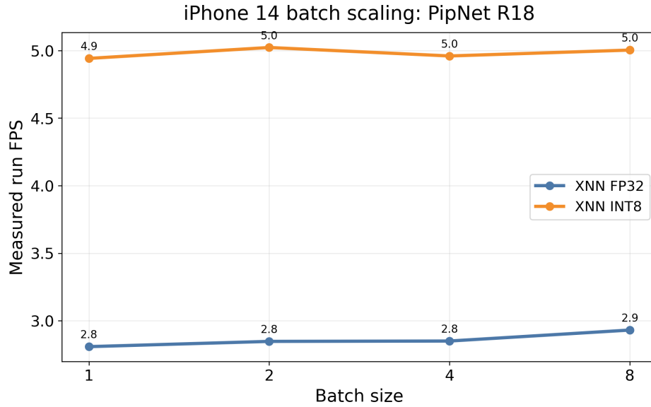
■ Figure 5.17 iPhone 14 batch scaling for PipNet ResNet18.
