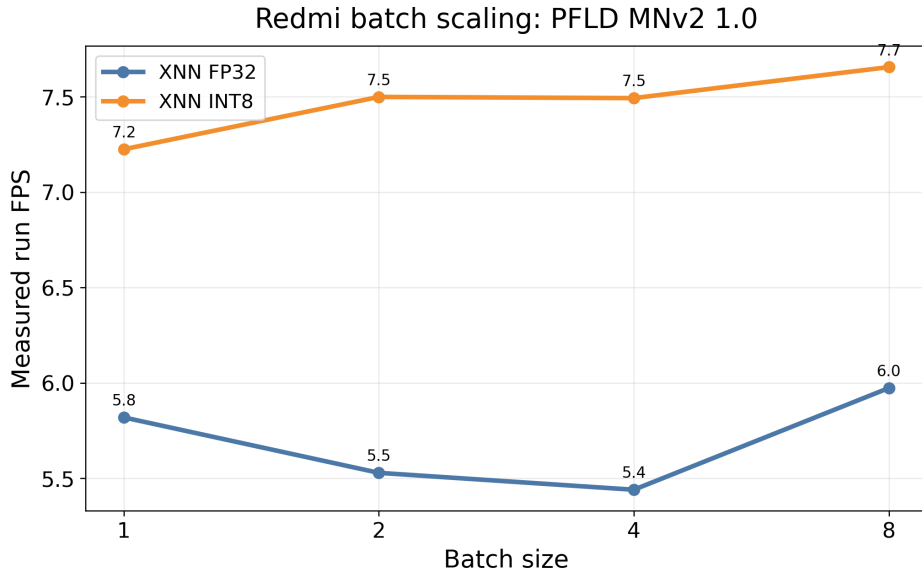
■ Figure 5.6 Focus device batch scaling for PFLD-MNv2-1.0 using XNNPACK variants.
