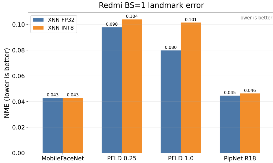
■ Figure 5.5 Focus device: BS=1 NME accuracy by backend and quantization (lower is better).
