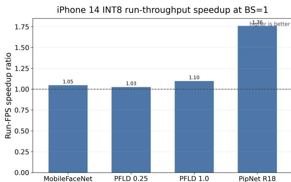
■ Figure 5.15 iPhone 14: INT8 and FP32 measured run-throughput comparison at BS=1.
