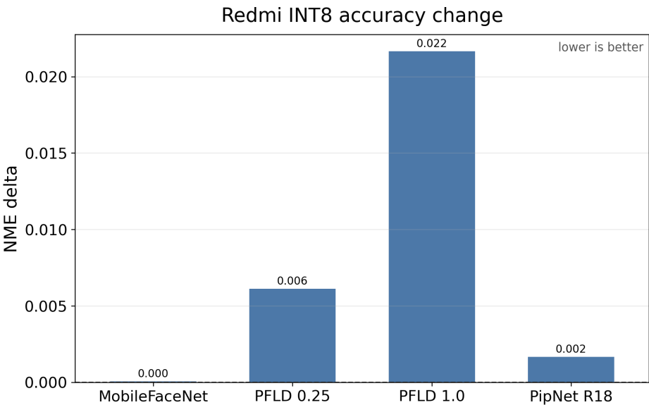
■ Figure 5.9 Focus device: INT8 vs FP32 NME difference at BS=1.
