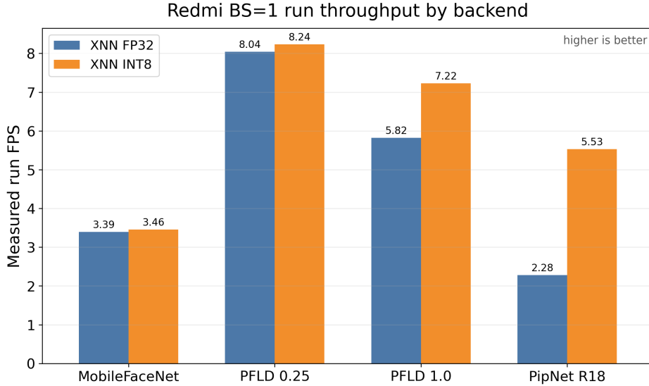
■ Figure 5.4 Focus device: BS=1 measured run throughput by backend and quantization.
