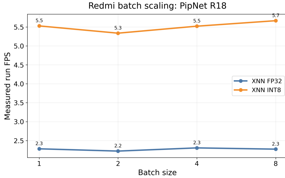
■ Figure 5.7 Focus device batch scaling for PipNet ResNet18 using XNNPACK variants.
