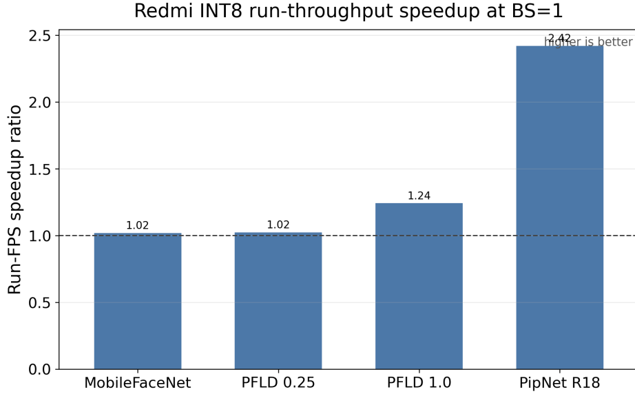
■ Figure 5.8 Focus device: INT8 vs FP32 measured run-throughput comparison at BS=1.
