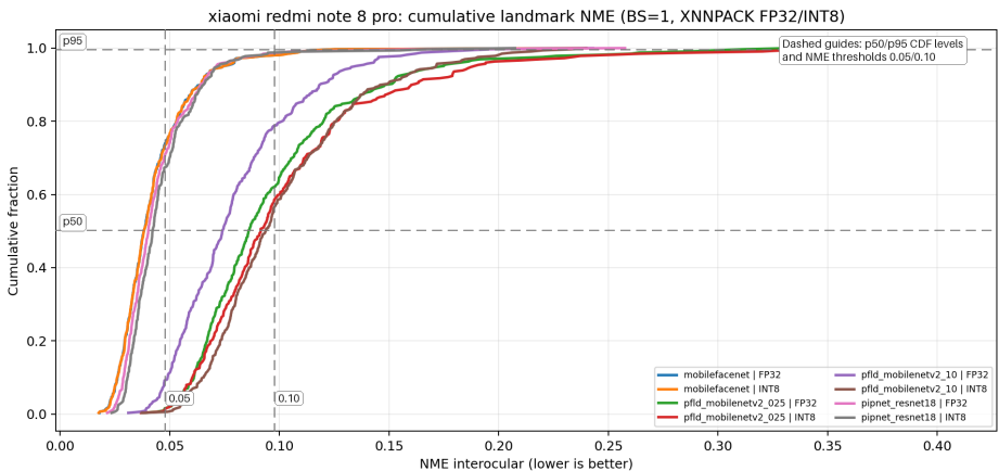
■ Figure 5.10 Focus device cumulative NME histogram for BS=1 XNNPACK FP32 and INT8 runs. Curves that rise earlier and stay higher indicate that more images have small normalized landmark error.
