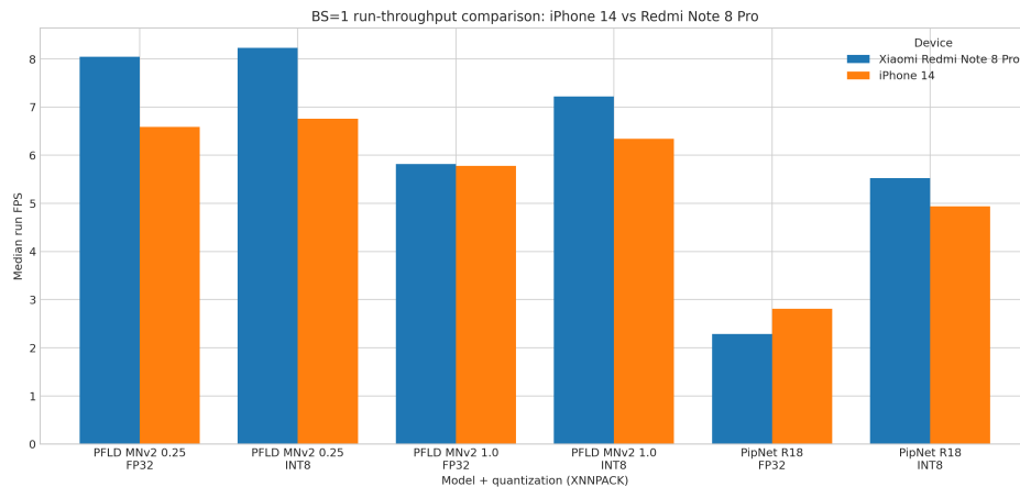
Figure 5.3 BS=1 XNNPACK measured run throughput on iPhone 14 and Redmi; higher run FPS is better.
