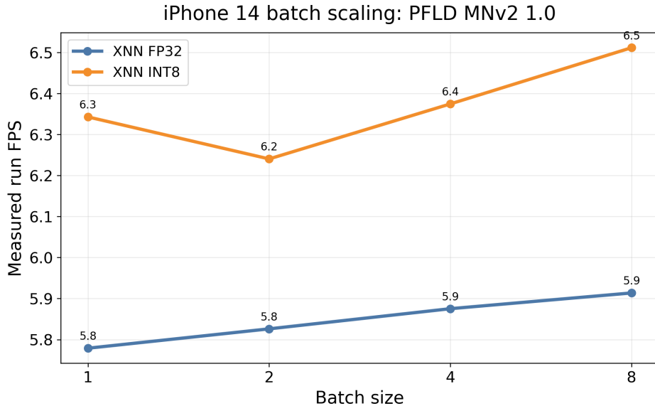
■ Figure 5.16 iPhone 14 batch scaling for PFLD-MNv2-1.0.
