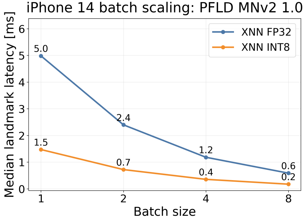
■ Figure 5.11 Per-image landmark-inference latency batch scaling on iPhone 14 for PFLD-MNv2-1.0. Total batch latency is divided by batch size.
