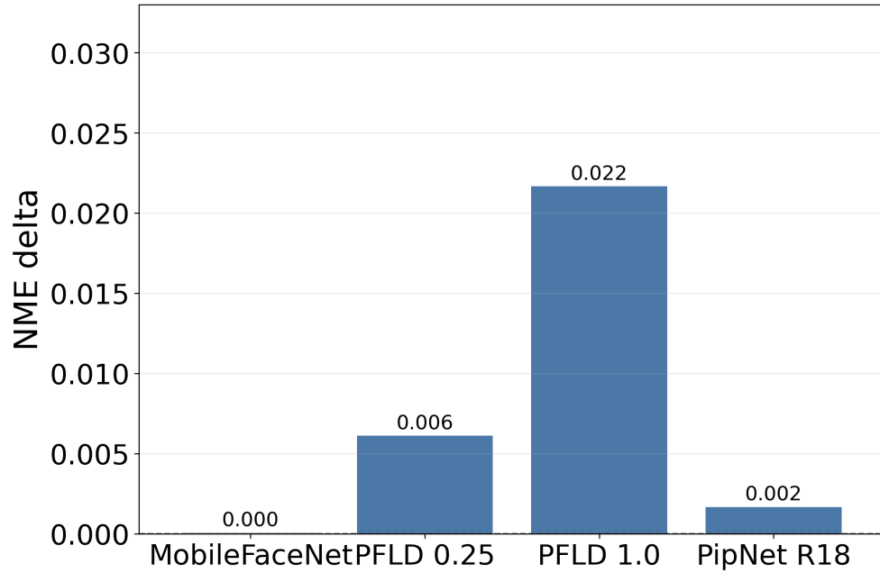
■ Figure 5.7 NME difference between INT8 and FP32 on Redmi at BS=1.
