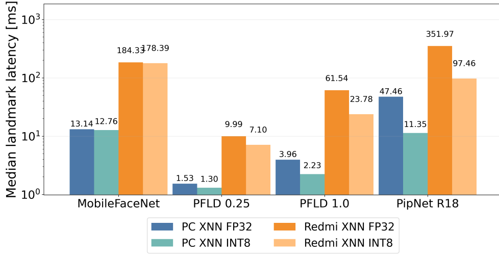
■ Figure 5.1 Landmark-inference latency at BS=1: PC vs Redmi median forward-pass time in milliseconds. Lower bars are better.
