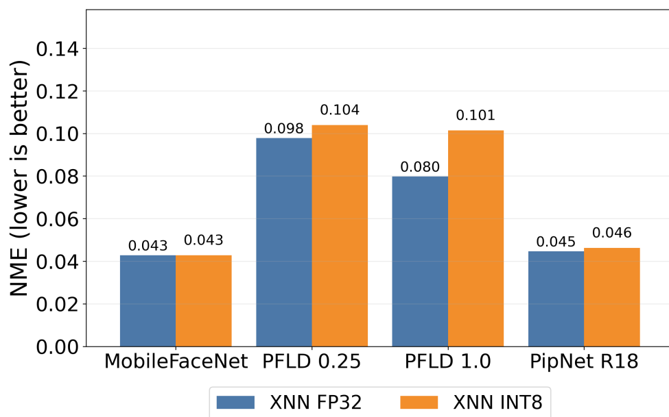
■ Figure 5.4 NME accuracy on Redmi at BS=1 by backend and quantization. Lower is better.
