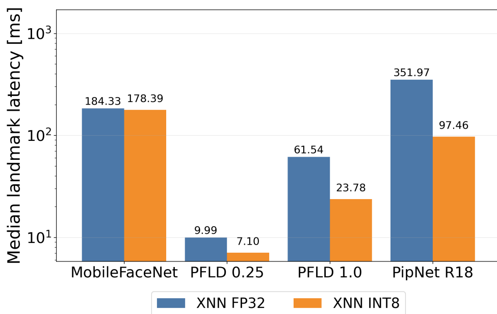
■ Figure 5.3 Landmark-inference latency on Redmi at BS=1 by backend and quantization. This chart focuses on the landmark model forward pass; lower latency is better.
