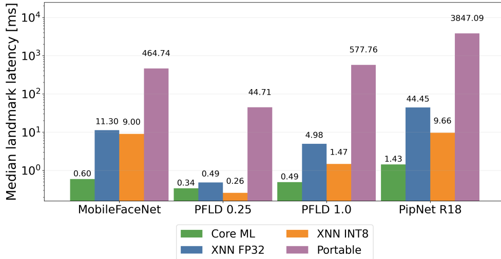
Figure 5.10 Landmark-inference latency on iPhone 14 at BS=1, reported as median forward-pass time.
