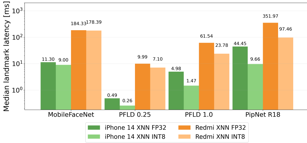
Figure 5.2 Landmark-inference latency at BS=1 with XNNPACK on iPhone 14 and Redmi. The chart uses only mobile devices and only the landmark forward pass; lower latency is better.
