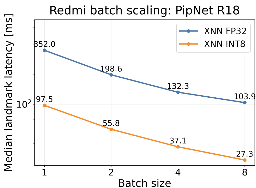
■ Figure 5.6 Per-image landmark-inference latency batch scaling on Redmi for PipNet ResNet18 using XNNPACK variants. Total batch latency is divided by batch size; lower latency is better.
