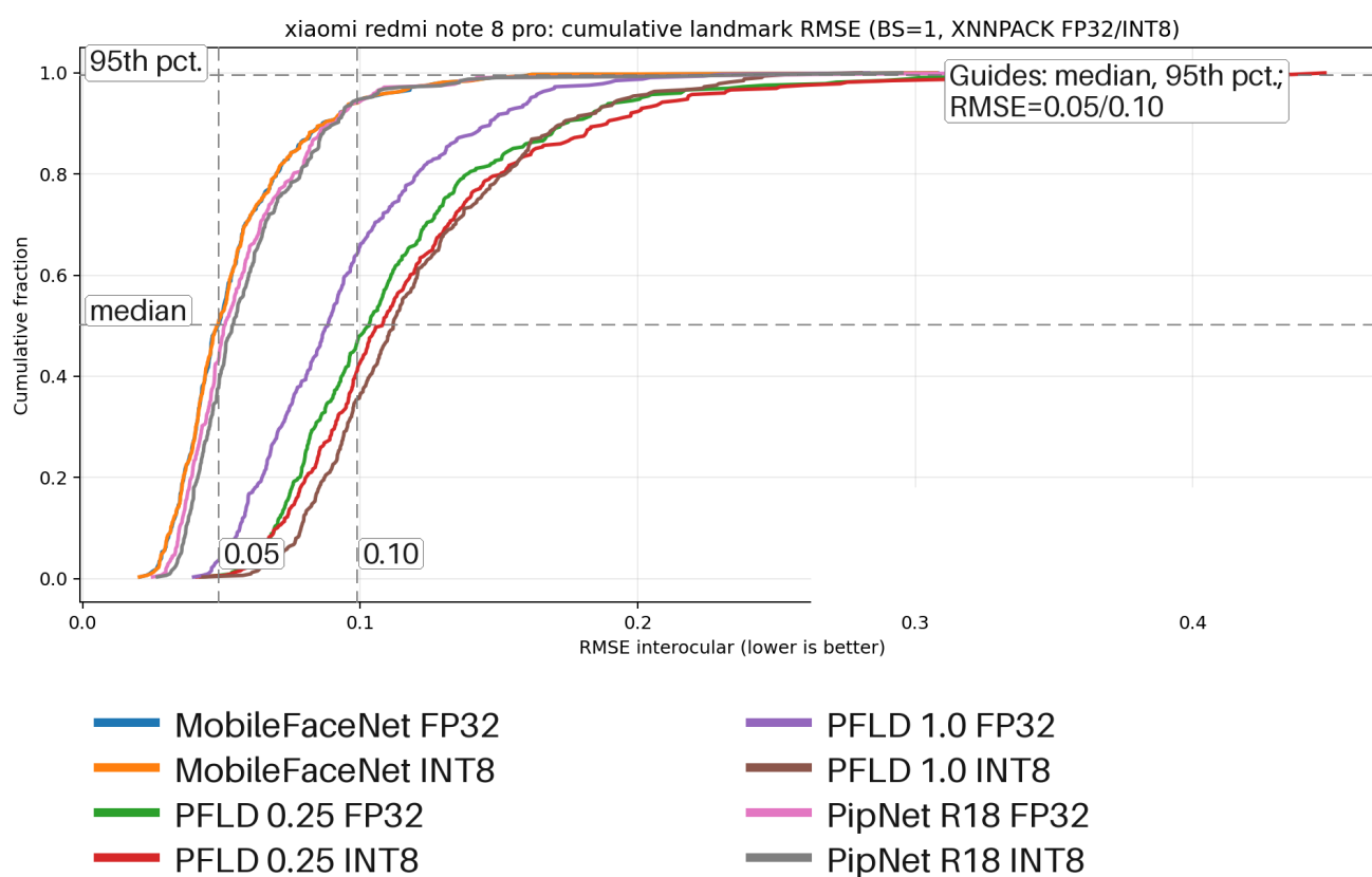
Figure 5.9 Cumulative RMSE histogram on Redmi for BS=1 XNNPACK FP32 and INT8 runs. This uses the same cumulative logic as the NME chart, but reports root-mean-square landmark error.
