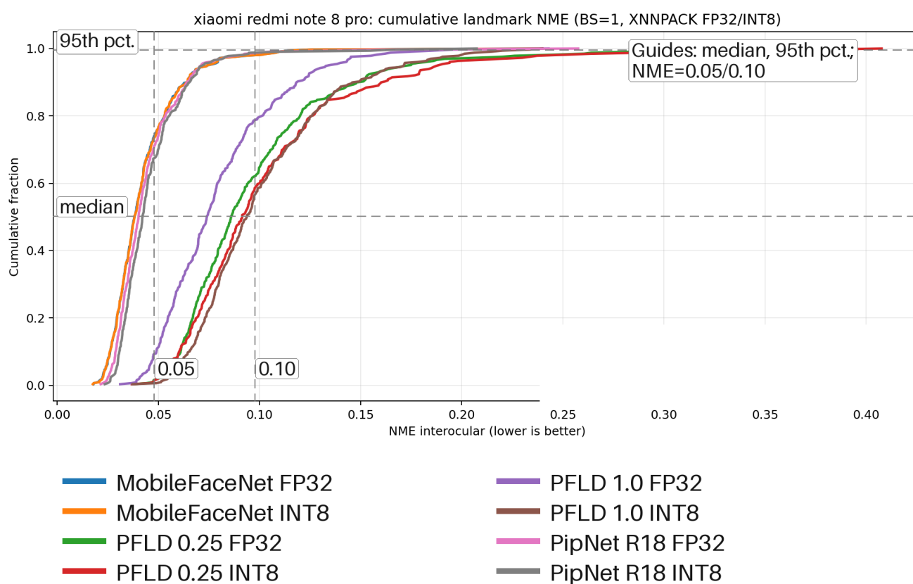
Figure 5.8 Cumulative NME histogram on Redmi for BS=1 XNNPACK FP32 and INT8 runs. Curves that rise earlier and stay higher indicate that more images have small normalized landmark error.
