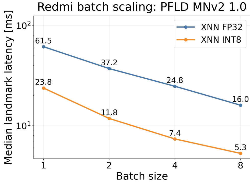
■ Figure 5.5 Per-image landmark-inference latency batch scaling on Redmi for PFLD-MNv2-1.0 using XNNPACK variants. Total batch latency is divided by batch size; lower latency is better.
