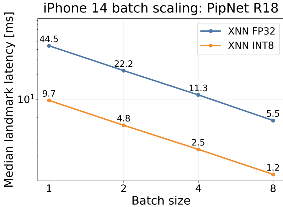
■ Figure 5.12 Per-image landmark-inference latency batch scaling on iPhone 14 for PipNet ResNet18. Total batch latency is divided by batch size.
