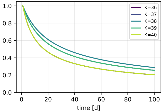
matrix CTF multiplier (WINJDAM, LINRAD)
