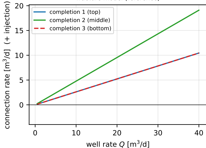
fracture model (reference)
