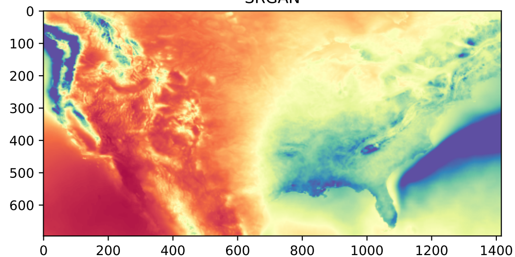
SRGAN
