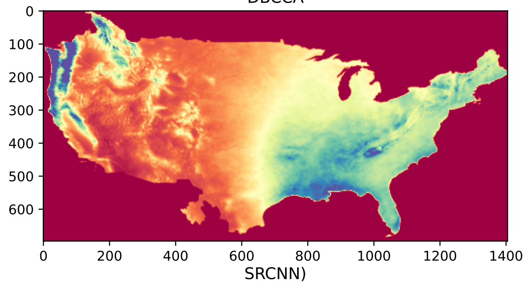
DBCCA
