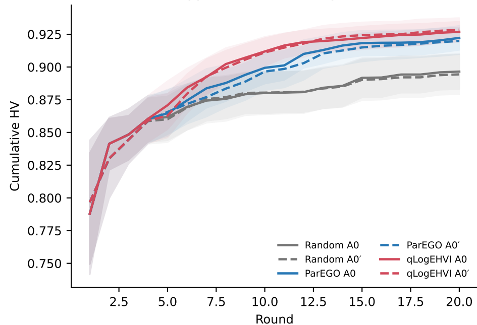
Hypervolume convergence
