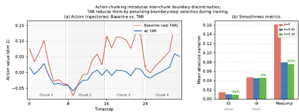
Fig. 1. Left: action trajectories across four consecutive chunks for the baseline (red) and a model trained with TAR (blue). Baseline transitions show abrupt velocity jumps; TAR produces smoother boundaries. Right: mean smoothness metrics (S1, IB, MaxJump) for three regularization strengths. Percentage labels show reduction relative to the baseline ( \lambda = 0 ).
