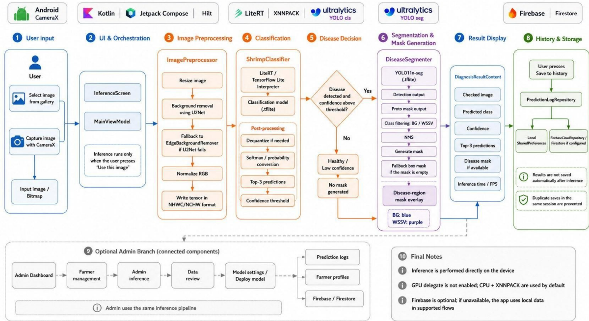
Fig. 5.1. Mobile AI pipeline from camera or gallery input through Android orchestration, image preprocessing, on-device classification, disease-conditioned segmentation, result presentation, history storage, and administrator-side review.
