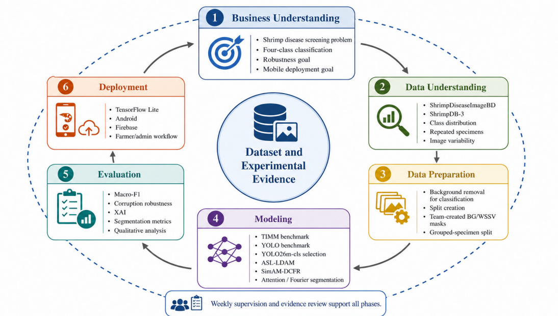
Fig. 2.2. CRISP-DM applied to the project.
